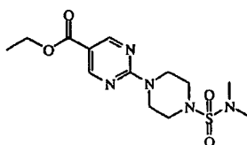
intermediate 3
